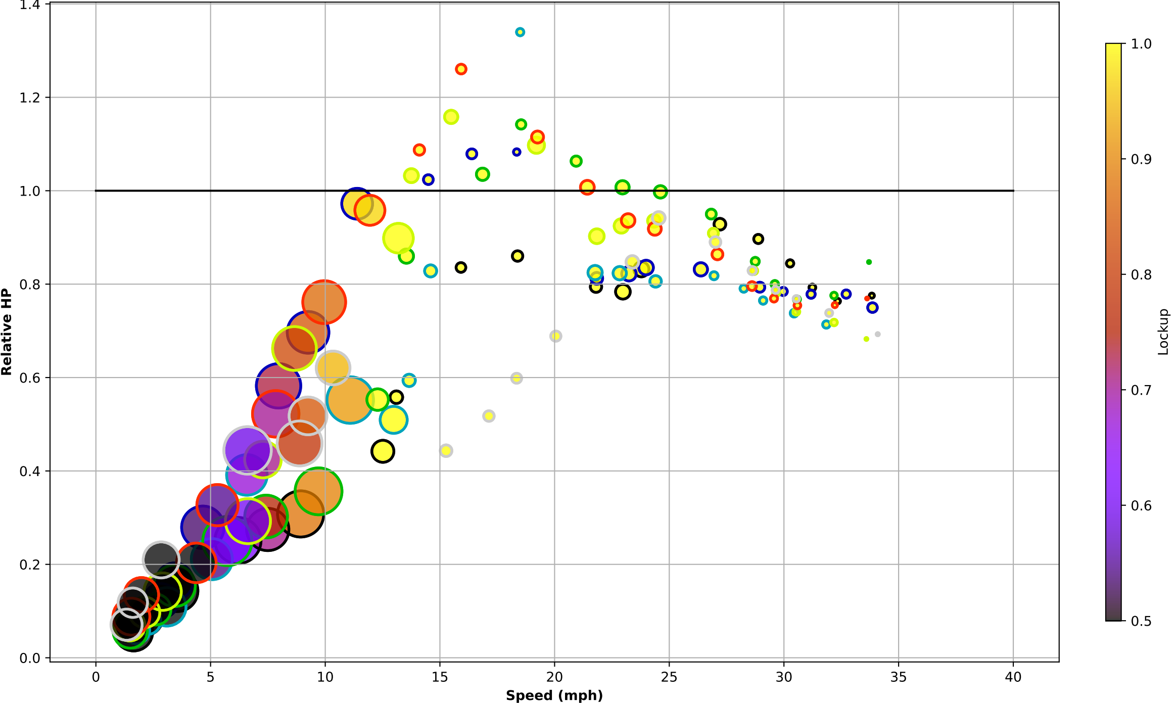
SAE Corrected HP Relative to Theoretical HP
